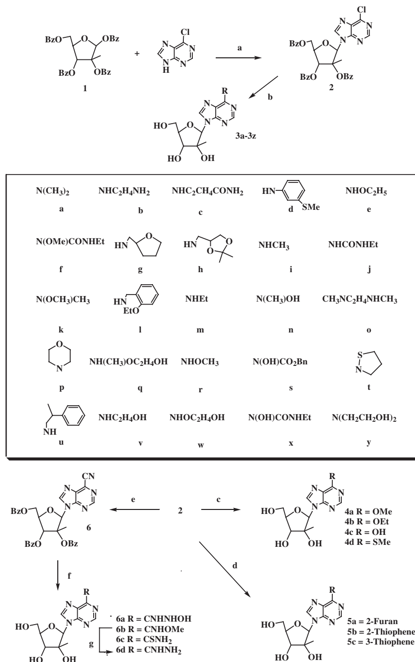
Scheme 1. (a) TMSOTf, BSA, \text{CH}_3\text{CN} , 60^\circ\text{C} , 3 h; (b) (i) amine, ethanol, 50^\circ\text{C} , 10 h; (ii) \text{NH}_3/\text{MeOH} or \text{NaCN}/\text{MeOH} , room temperature, 12 h; (c) \text{NaOMe} or \text{NaOEt} or \text{NaOH} or \text{NaSMe} , ethanol, 50^\circ\text{C} , 4 h; (d) (i) \text{Pd}(\text{PPh}_3)_4 , \text{K}_2\text{CO}_3 , toluene, \text{RB}(\text{OH})_2 , 100^\circ\text{C} , 12 h; (ii) \text{NH}_3/\text{MeOH} , room temperature, 10 h; (e) \text{Pd}(\text{PPh}_3)_4 , \text{Zn}(\text{CN})_2 , toluene, 80^\circ\text{C} , 10 h; (f) (i) \text{NH}_2\text{OH} or \text{NaCN}/\text{MeOH} or \text{H}_2\text{S} ; (ii) \text{NH}_3/\text{MeOH} , room temperature, 10 h; (g) \text{NH}_4\text{Cl} , \text{MeOH} , 70^\circ\text{C} , 15 h.
