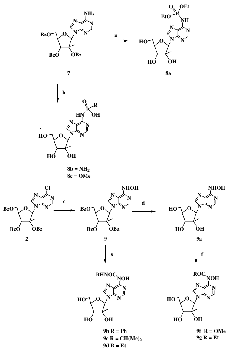
Scheme 2. (a) (i) \text{POCl}_3 , 1,2,4-triazole, triethylamine, \text{CH}_3\text{CN} , 0^\circ\text{C} , 30 min; (ii) 7 , pyridine, room temperature; 1 h; (iii) ethanol, room temperature, 1 h; (iv) \text{NaCN} , \text{MeOH} , 15% overall yield; (b) (i) \text{POCl}_3 , 1,2,4-triazole, triethylamine, \text{CH}_3\text{CN} , 0^\circ\text{C} , 30 min; (ii) 7 , pyridine, room temperature; 1 h; (iii) triethylammonia carbonate, room temperature, 1 h; (iv) \text{NH}_3/\text{MeOH} ; (c) \text{NH}_2\text{OH} , room temperature, 10 h; (d) \text{NaCN}/\text{MeOH} , room temperature, 12 h; (e) (i) (\text{Me})_2\text{CHNCO} or \text{EtNCO} or \text{PhNCO} , \text{CHCl}_3 , 40^\circ\text{C} , 10 h; (ii) \text{NaCN}/\text{MeOH} , room temperature, 12 h; (f) (i) TMSI, 1,2,4-triazole, pyridine, room temperature, 4 h; (ii) \text{C}_2\text{H}_5\text{COCl} or \text{CH}(\text{OMe})_3 , pyridine, room temperature, 10 h; (iii) \text{NH}_4\text{OH} .
