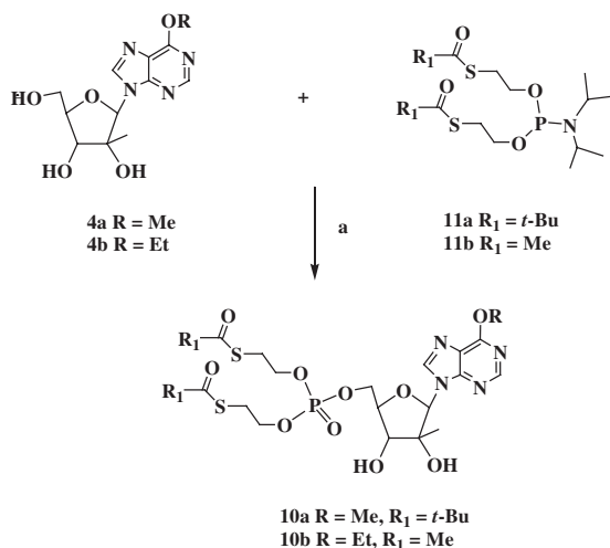
Scheme 3. (a) (i) Tetrazole; (ii) t -BuOOH, DMF.
